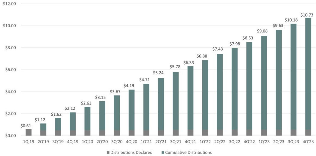
Cumulative Distributions 1
